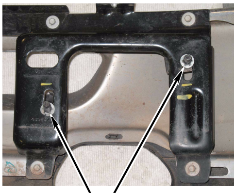
Bumper mounting bolts (captive) on the bumper mounting bracket
