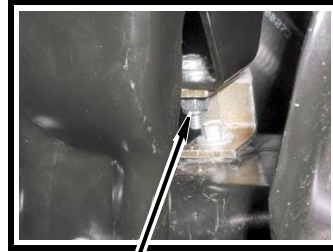
Kit Bolt (1/4" x 1"), Washer (1/4"), Nut (1/4" Nylock)
