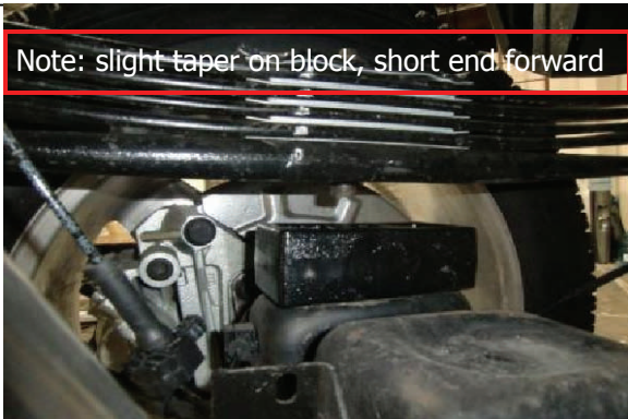
Locate lift block on axle mount and raise to meet leaf spring
