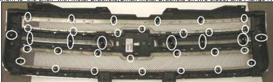
Figure 3 – Rear view of vehicle's shell; Grills attached with Metal Brackets and Flange Nuts
