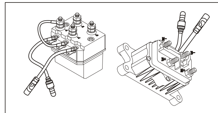
Figure 5. Contactors for ATV winch
