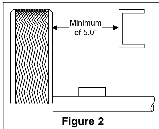
Before starting this installation, carefully measure the distance between the frame and inner part of the tire when vehicle is at normal height.
