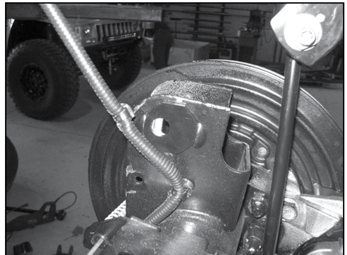
Fig. 2B - Shows Highest Pinion Angle Position
