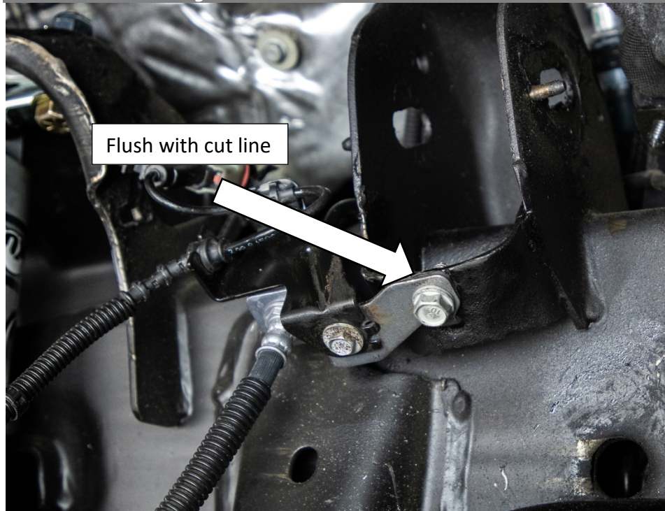
Figure 8: Reinstall Brake Line Bracket
