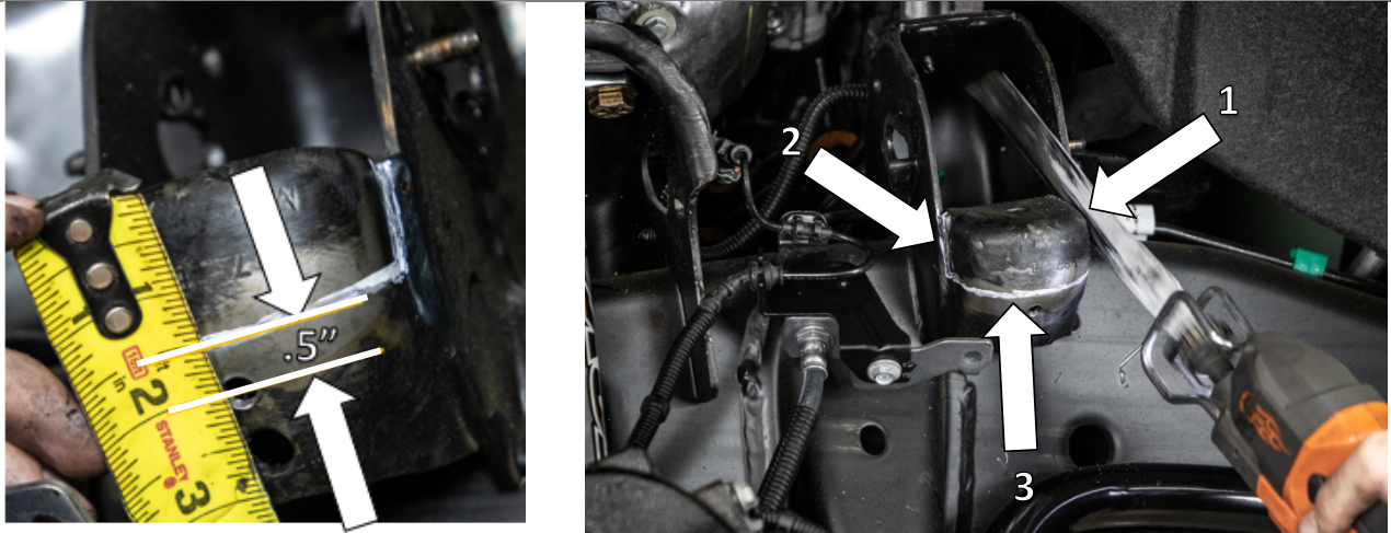
Figure 7: Mark and Cut the Service Perch
