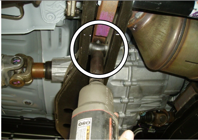
Figure 1: Torsion Bar Adjusting Screw
