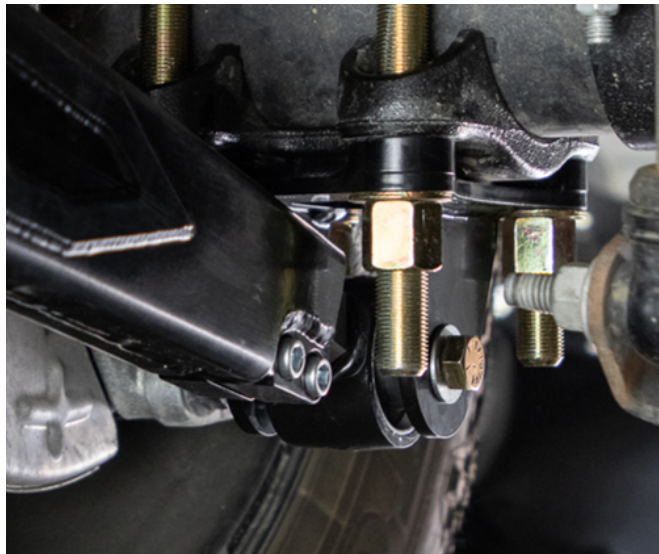
Figure 17: Traction Bar and Axle Mount Installation
