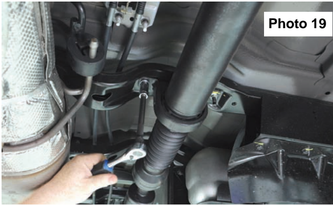
Lower the carrier bearing.
