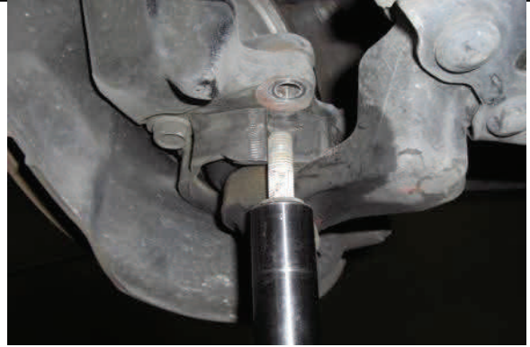
Disconnect lower ball joint hardware bolts
