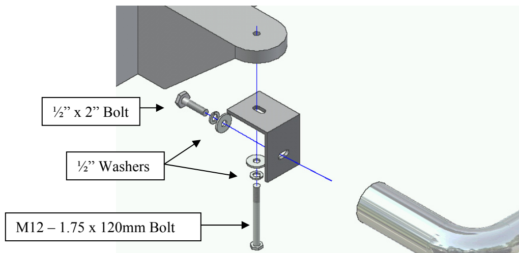
Figure 1.2 – Front Bracket
