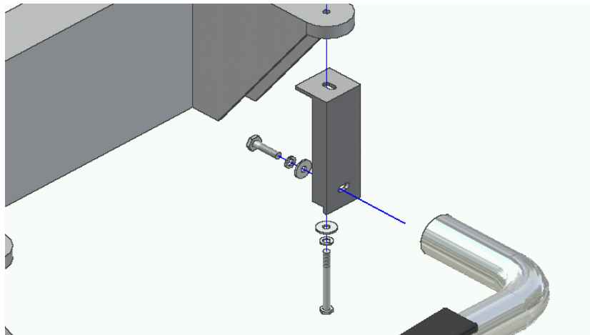
Figure 1.4 – Rear Bracket
