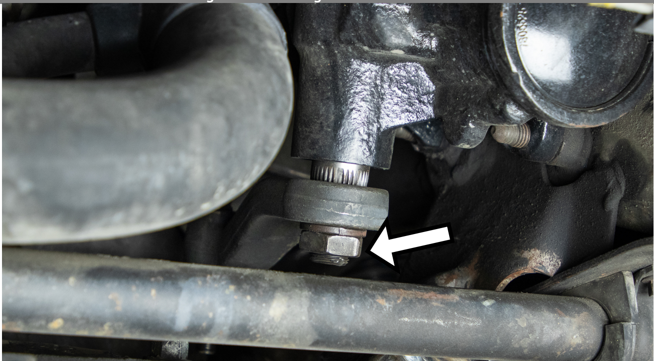
Figure 3: Unbolting Pitman Arm Bracket
