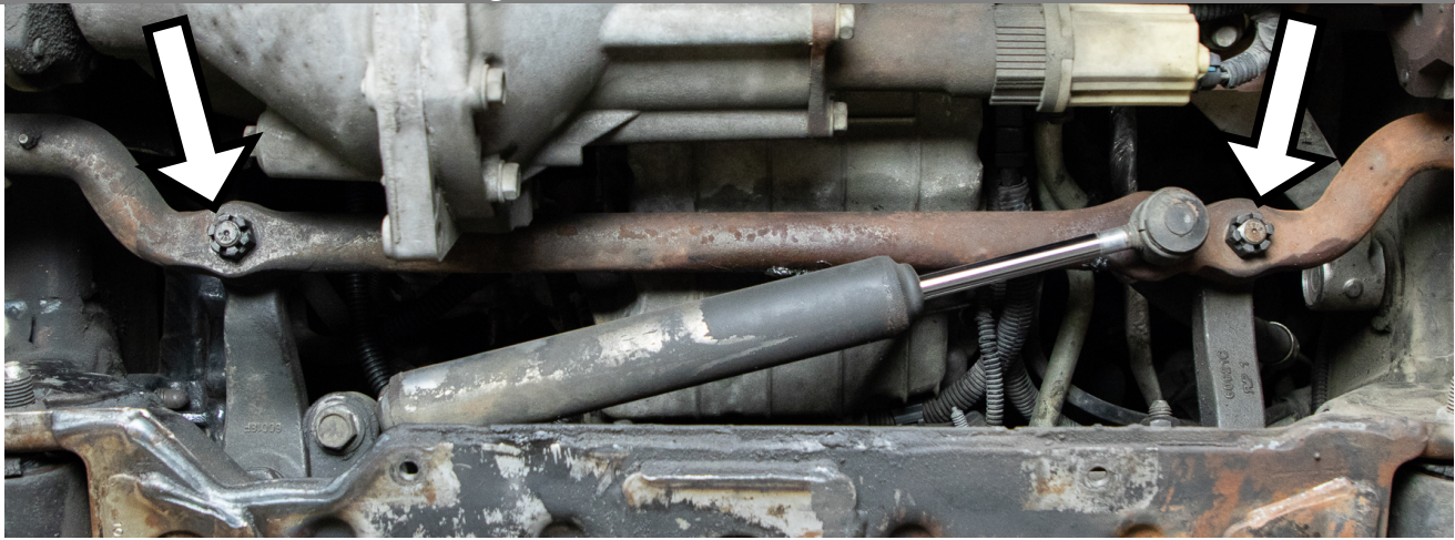
Figure 2: Pitman and Idler Arm Nuts
