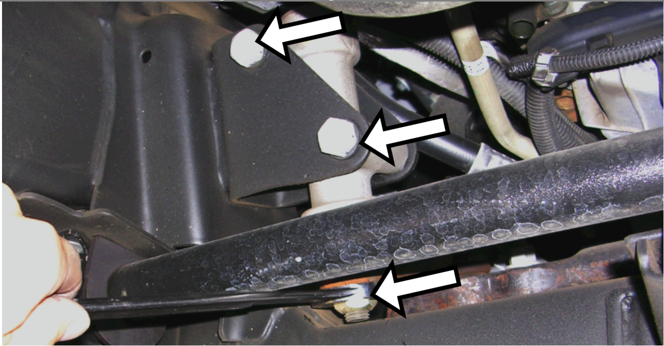
Figure 4: Removing the Idler Arm Nut
