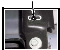
Bumper Bracket (passenger side)
