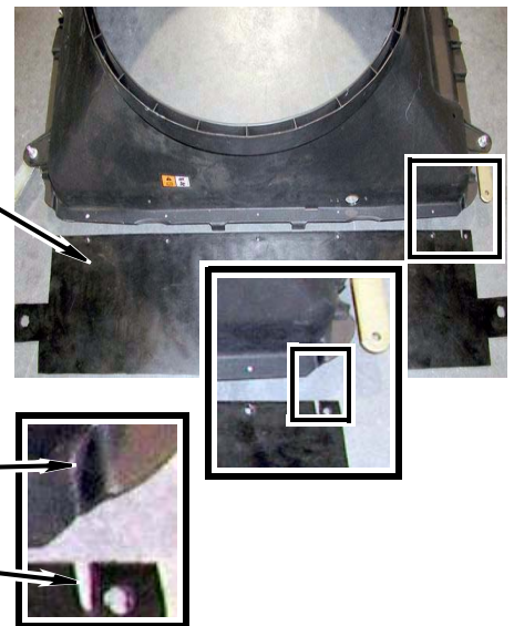
Kit Gap Guard
